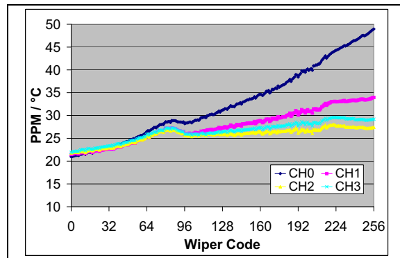
FIGURE 2-39: 10 kΩ – R_{BW} PPM/°C vs. Wiper Setting. ( R_{BW}(\text{code}=n, 125^\circ\text{C}) - R_{BW}(\text{code}=n, -40^\circ\text{C}) ) / R_{BW}(\text{code}=256, 25^\circ\text{C}) / 165^\circ\text{C} * 1,000,000 ) ( V_{DD} = 5.5\text{V} , I_W = 150\text{ }\mu\text{A} ).
