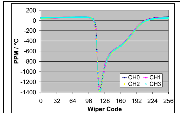
FIGURE 2-40: 10 kΩ – R_{BW} PPM/°C vs. Wiper Setting. ( R_{BW}(\text{code}=n, 125^\circ\text{C}) - R_{BW}(\text{code}=n, -40^\circ\text{C}) ) / R_{BW}(\text{code}=256, 25^\circ\text{C}) / 165^\circ\text{C} * 1,000,000 ) ( V_{DD} = 3.0\text{V} , I_W = 150\text{ }\mu\text{A} ).
