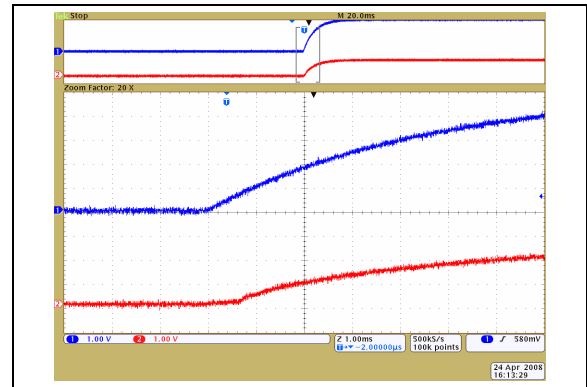
FIGURE 2-64: 50 k \Omega – Low-Voltage Increment Wiper Settling Time ( V_{DD} = 2.7\text{V} ) (1 \mu\text{s}/\text{Div} ).
