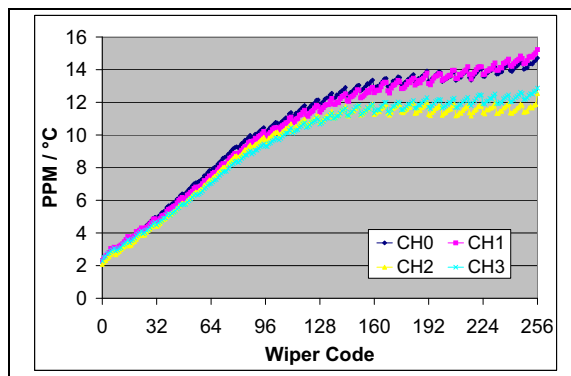
FIGURE 2-79: 100 k \Omega – R_{WB} PPM/ ^\circ\text{C} vs. Wiper Setting. ( R_{BW(\text{code}=n, 125^\circ\text{C})} - R_{BW(\text{code}=n, -40^\circ\text{C})} / R_{BW(\text{code}=256, 25^\circ\text{C})} / 165^\circ\text{C} * 1,000,000 ) ( V_{DD} = 5.5\text{V} , I_W = 45\text{ }\mu\text{A} ).
