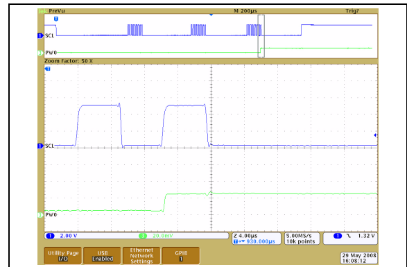
FIGURE 2-65: 50 k \Omega – Low-Voltage Increment Wiper Settling Time ( V_{DD} = 5.5\text{V} ) (1 \mu\text{s}/\text{Div} ).
