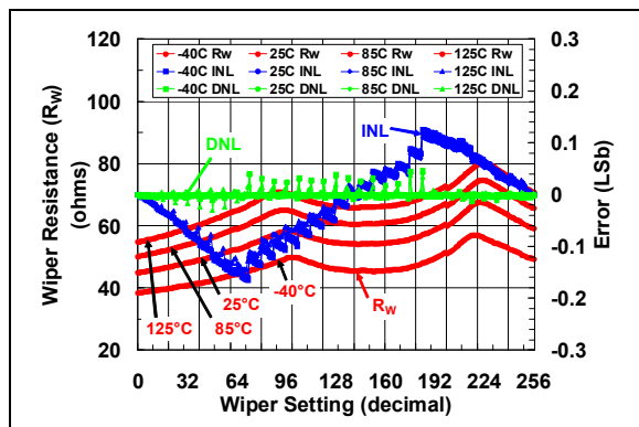
FIGURE 2-46: 50 k \Omega Pot Mode – R_W ( \Omega ), INL (LSb), DNL (LSb) vs. Wiper Setting and Ambient Temperature ( V_{DD} = 5.5\text{V} ).
