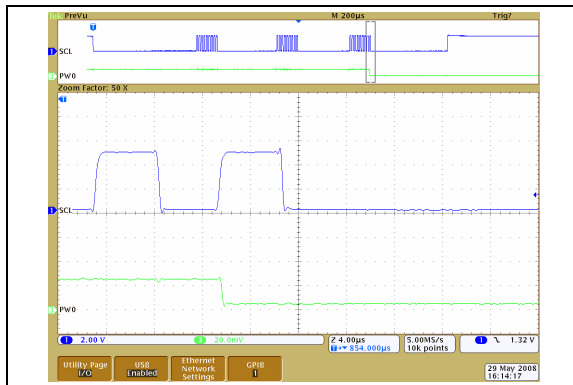
FIGURE 2-63: 50 kΩ – Low-Voltage Decrement Wiper Settling Time ( V_{DD} = 5.5\text{V} ) (1 μs/Div).
