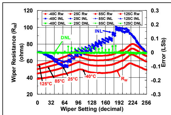
FIGURE 2-49: 50 k \Omega Rheo Mode – R_W ( \Omega ), INL (LSb), DNL (LSb) vs. Wiper Setting and Ambient Temperature ( V_{DD} = 5.5\text{V} ).
