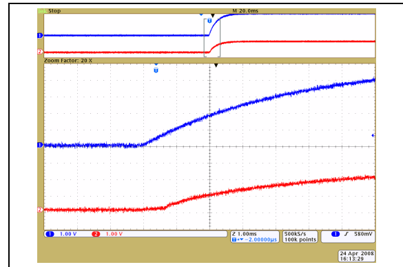
FIGURE 2-64: 50 kΩ – Low-Voltage Increment Wiper Settling Time ( V_{DD} = 2.7\text{V} ) (1 μs/Div).
