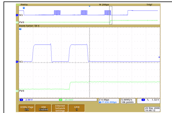
FIGURE 2-65: 50 kΩ – Low-Voltage Increment Wiper Settling Time ( V_{DD} = 5.5\text{V} ) (1 μs/Div).
