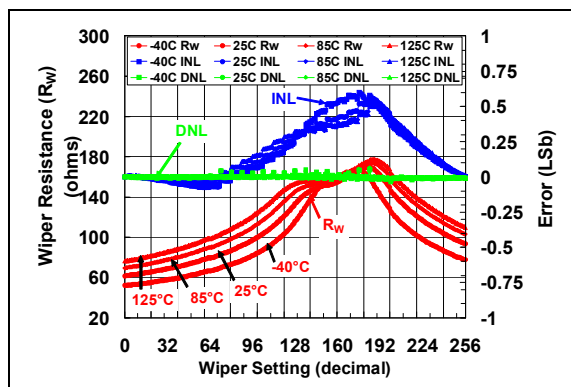
FIGURE 2-50: 50 k \Omega Rheo Mode – R_W ( \Omega ), INL (LSb), DNL (LSb) vs. Wiper Setting and Ambient Temperature ( V_{DD} = 3.0\text{V} ).
