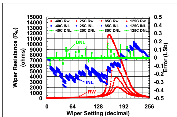
FIGURE 2-47: 50 k \Omega Pot Mode – R_W ( \Omega ), INL (LSb), DNL (LSb) vs. Wiper Setting and Ambient Temperature ( V_{DD} = 3.0\text{V} ).
