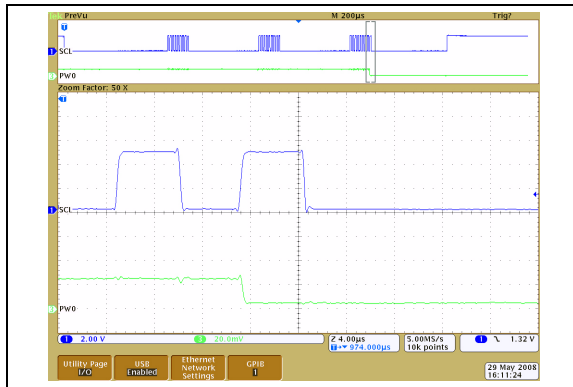
FIGURE 2-62: 50 kΩ – Low-Voltage Decrement Wiper Settling Time ( V_{DD} = 2.7\text{V} ) (1 μs/Div).
