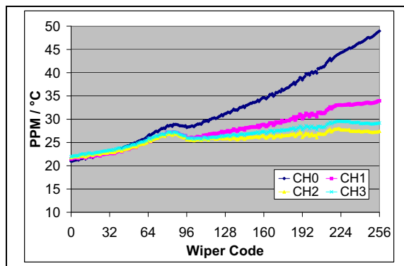
FIGURE 2-39: 10 kΩ – R_{BW} PPM/°C vs. Wiper Setting. ( R_{BW}(\text{code}=n, 125^\circ\text{C}) - R_{BW}(\text{code}=n, -40^\circ\text{C}) ) / R_{BW}(\text{code}=256, 25^\circ\text{C}) / 165^\circ\text{C} * 1,000,000 ) ( V_{DD} = 5.5\text{V} , I_W = 150\text{ }\mu\text{A} ).
