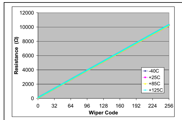
FIGURE 2-33: 10 kΩ – R_{WB} (Ω) vs. Wiper Setting and Ambient Temperature ( V_{DD} = 5.5\text{V} , I_W = 150\text{ μA} ).
