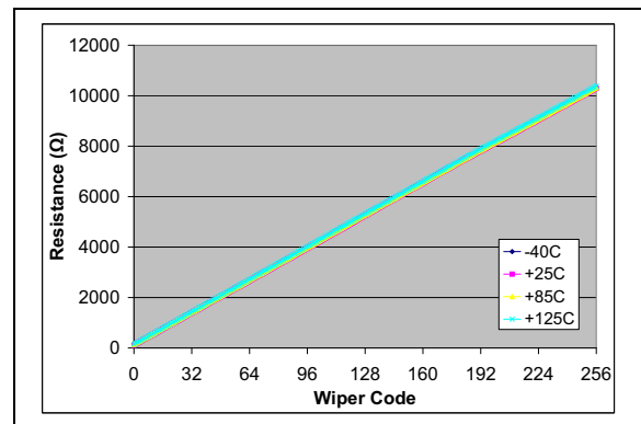
FIGURE 2-34: 10 kΩ – R_{WB} (Ω) vs. Wiper Setting and Ambient Temperature ( V_{DD} = 3.0\text{V} , I_W = 150\text{ μA} ).
