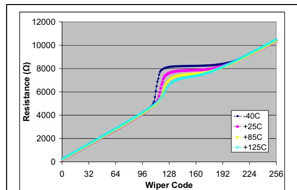
FIGURE 2-34: 10 kΩ – R_{WB} (Ω) vs. Wiper Setting and Ambient Temperature ( V_{DD} = 3.0\text{V} , I_W = 150\text{ μA} ).
