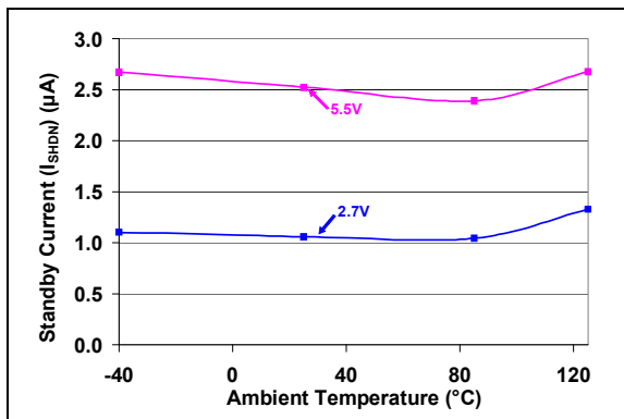
FIGURE 2-2: Device Current ( I_{\text{SHDN}} ) and V_{DD} . (HVC/A0 = V_{DD} ) vs. Ambient Temperature.
