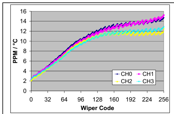
FIGURE 2-79: 100 kΩ – R_{WB} PPM/ ^\circ\text{C} vs. Wiper Setting. ( R_{BW}(\text{code}=n, 125^\circ\text{C}) - R_{BW}(\text{code}=n, -40^\circ\text{C}) / R_{BW}(\text{code}=256, 25^\circ\text{C}) / 165^\circ\text{C} * 1,000,000 ) ( V_{DD} = 5.5\text{V} , I_W = 45\text{ }\mu\text{A} ).
