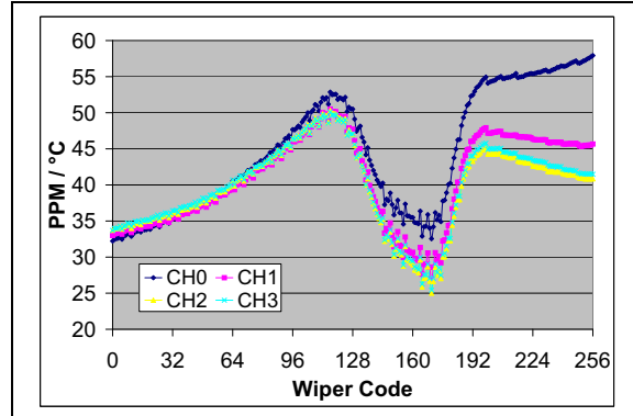
FIGURE 2-40: 10 kΩ – R_{BW} PPM/°C vs. Wiper Setting. ( R_{BW}(\text{code}=n, 125^\circ\text{C}) - R_{BW}(\text{code}=n, -40^\circ\text{C}) ) / R_{BW}(\text{code} = 256, 25^\circ\text{C}) / 165^\circ\text{C} * 1,000,000 ) ( V_{DD} = 3.0\text{V} , I_W = 150\text{ }\mu\text{A} ).
