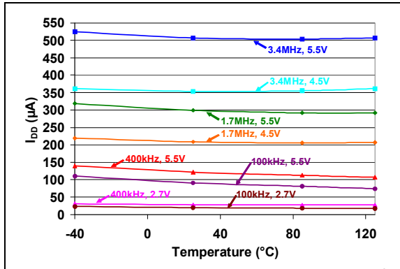
FIGURE 2-1: Device Current ( I_{DD} ) vs. I^2\text{C} Frequency ( f_{SCL} ) and Ambient Temperature ( V_{DD} = 2.7\text{V} and 5.5\text{V} ).
