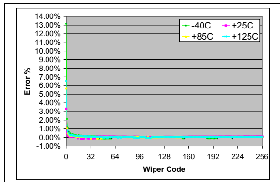
FIGURE 2-76: 100 k \Omega – Worst Case R_{BW} from Average R_{BW} ( R_{BW0} - R_{BW3} ) Error (%) vs. Wiper Setting and Temperature ( V_{DD} = 5.5\text{V} , I_W = 45\text{ }\mu\text{A} ).
