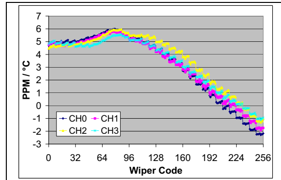
FIGURE 2-59: 50 kΩ – R_{WB} PPM/°C vs. Wiper Setting. ( R_{BW}(\text{code}=n, 125^\circ\text{C}) - R_{BW}(\text{code}=n, -40^\circ\text{C}) ) / R_{BW}(\text{code} = 256, 25^\circ\text{C}) / 165^\circ\text{C} * 1,000,000 ) ( V_{DD} = 5.5\text{V} , I_W = 90\text{ }\mu\text{A} ).
