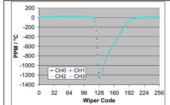
FIGURE 2-60: 50 kΩ – R_{WB} PPM/°C vs. Wiper Setting. ( R_{BW}(\text{code}=n, 125^\circ\text{C}) - R_{BW}(\text{code}=n, -40^\circ\text{C}) ) / R_{BW}(\text{code} = 256, 25^\circ\text{C}) / 165^\circ\text{C} * 1,000,000 ) ( V_{DD} = 3.0\text{V} , I_W = 48\text{ }\mu\text{A} ).
