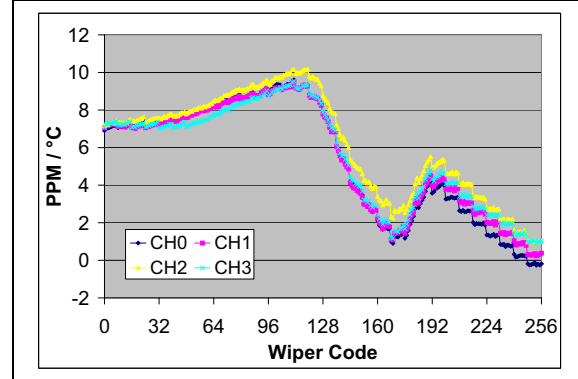
FIGURE 2-60: 50 kΩ – R_{WB} PPM/°C vs. Wiper Setting. ( R_{BW}(\text{code}=n, 125^\circ\text{C}) - R_{BW}(\text{code}=n, -40^\circ\text{C}) ) / R_{BW}(\text{code} = 256, 25^\circ\text{C}) / 165^\circ\text{C} * 1,000,000 ) ( V_{DD} = 3.0\text{V} , I_W = 48\text{ }\mu\text{A} ).
