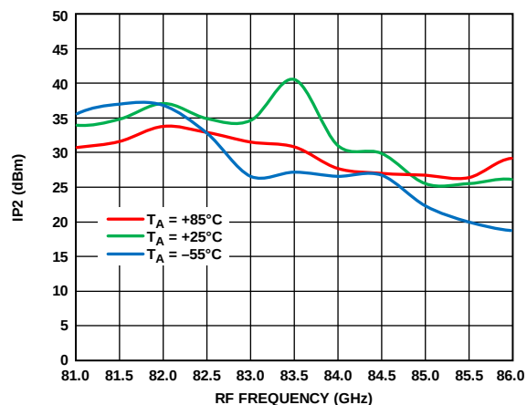
Figure 187. Input IP2 vs. RF Frequency at Various Temperatures, R_{FIN} = -20 dBm, LO = 2 dBm, IF = 2000 MHz, V_{DLNA} = 3 V
