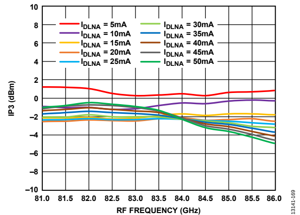
Figure 157. Input IP3 vs. RF Frequency at Various I_{DLNA} Values, R_{FIN} = -20 dBm, LO = 2 dBm, IF = 1000 MHz, V_{DLNA} = 3 V
