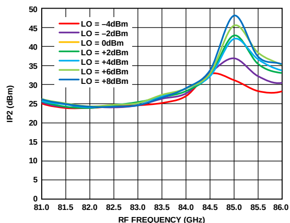
Figure 188. Input IP2 vs. RF Frequency at Various LO Powers, R_{FIN} = -20 dBm, IF = 2000 MHz, V_{DLNA} = 3 V
