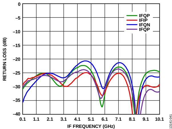
Figure 41. IF Return Loss vs. IF Frequency, LO = 2 dBm at 12 GHz, V_{DLNA} = 3\text{ V}
