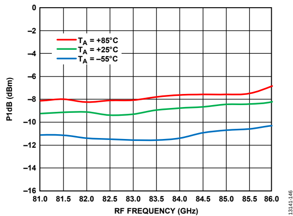
Figure 138. Input P1dB vs. RF Frequency at Various Temperatures, LO = 2 dBm, IF = 500 MHz, V_{DLN} = 4\text{ V}
