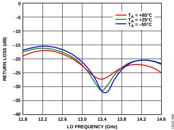
Figure 40. LO Return Loss vs. LO Frequency at Various Temperatures, LO = 2 dBm, V_{DLNA} = 3\text{ V}
