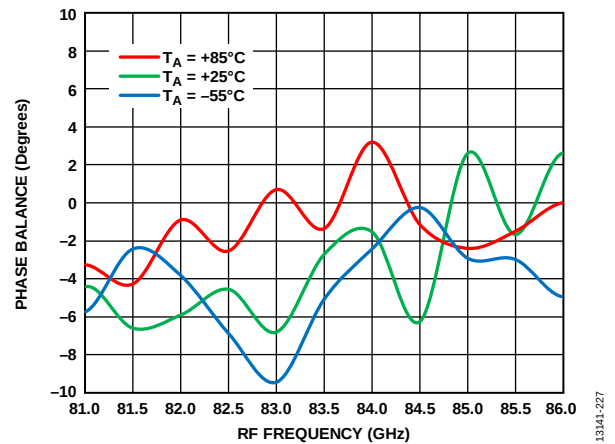
Figure 207. Phase Balance vs. RF Frequency at Various Temperatures, RFIN = -20 dBm, LO = 2 dBm, IF = 500 MHz, V DLNA = 3 V
