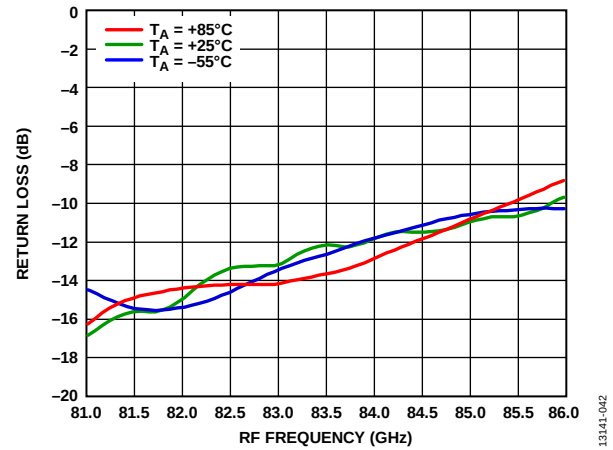
Figure 42. RF Return Loss vs. RF Frequency at Various Temperatures, LO = 2 dBm, LO = 12 GHz, V_{DLNA} = 3\text{ V}
