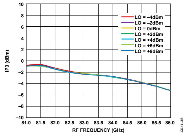
Figure 156. Input IP3 vs. RF Frequency at Various LO Powers, R_{FIN} = -20 dBm, IF = 1000 MHz, V_{DLNA} = 3 V
