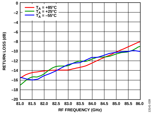
Figure 39. RF Return Loss vs. RF Frequency at Various Temperatures, LO = 2 dBm, LO = 12 GHz, V_{DLNA} = 4\text{ V}
