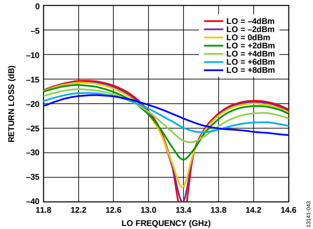
Figure 43. LO Return Loss vs. LO Frequency at Various LO Powers, V_{DLNA} = 3\text{ V}
