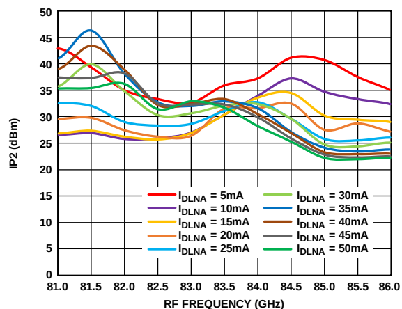
Figure 189. Input IP2 vs. RF Frequency at Various I_{DLNA} Values, R_{FIN} = -20 dBm, LO = 2 dBm, IF = 2000 MHz, V_{DLNA} = 3 V
