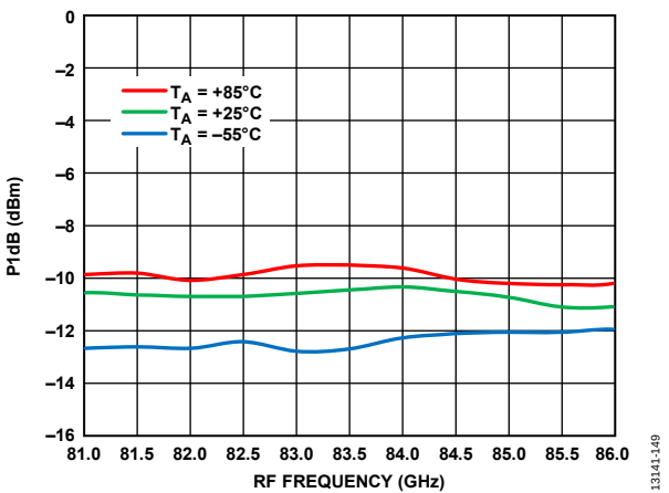
Figure 139. Input P1dB vs. RF Frequency at Various Temperatures, LO = 2 dBm, IF = 500 MHz, V_{DLN} = 3\text{ V}
