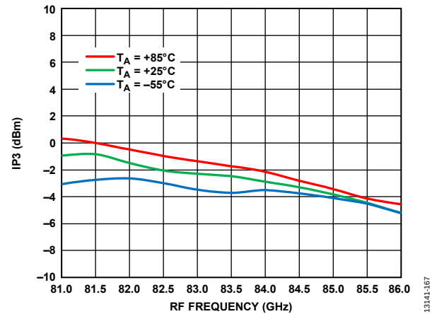
Figure 155. Input IP3 vs. RF Frequency at Various Temperatures, R_{FIN} = -20 dBm, LO = 2 dBm, IF = 1000 MHz, V_{DLNA} = 3 V
