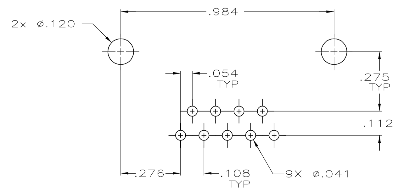
P.C. BOARD MOUNTING DIMENSIONS \Delta
