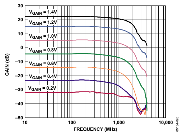
Figure 26. Gain vs. Frequency (Using ETC1-13 Baluns)
