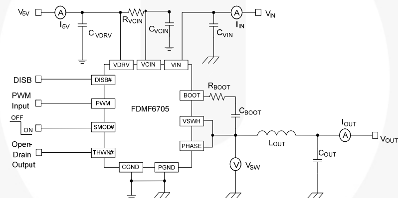
Figure 28. Power Loss Measurement Block Diagram
