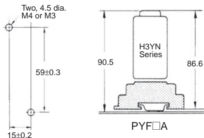
Mounting Holes
