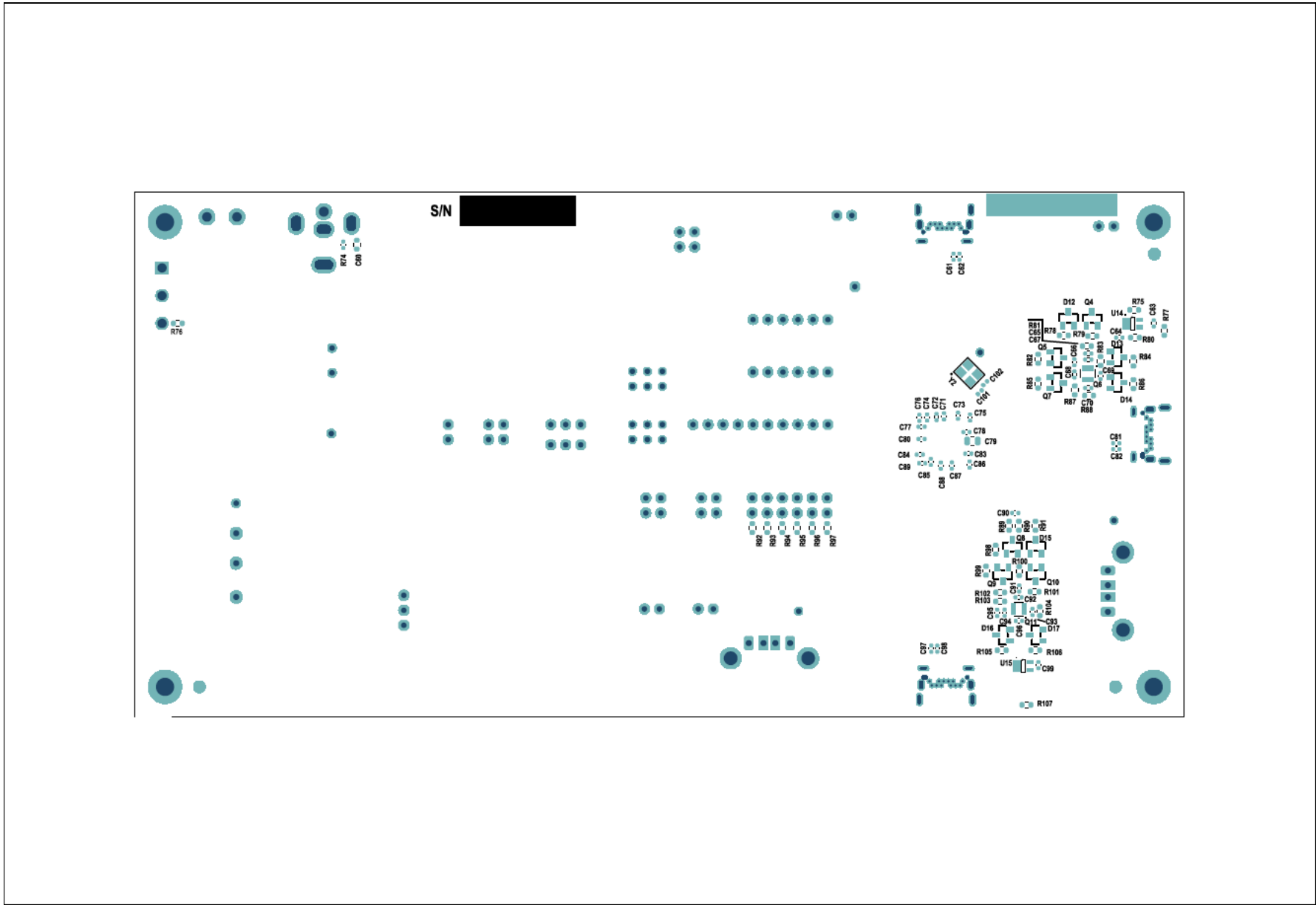
FIGURE C-2: EVB-USB7002 BOTTOM SILK SCREEN IMAGE
