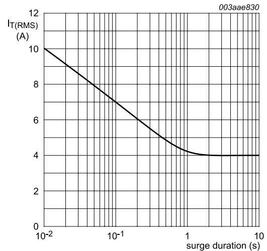
f = 50 Hz; T_{mb} \leq 107 °C Fig. 2. RMS on-state current as a function of surge duration; maximum values
