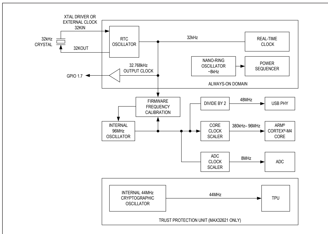
Figure 1. Clock Diagram
