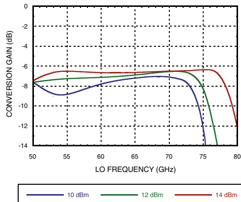
Conversion Gain vs. LO Power IF= 10 GHz
