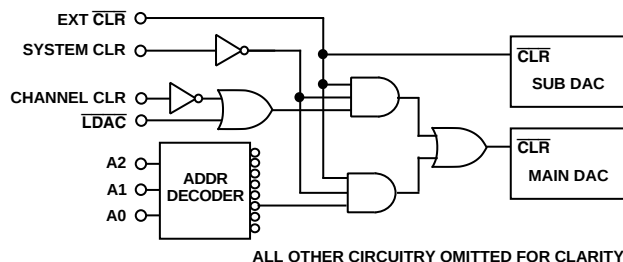
Figure 20. \overline{\text{CLR}} Functions for Main and Sub DACs
