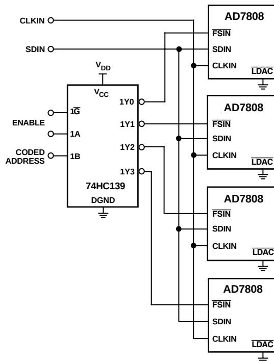
Figure 42. Decoding Multiple AD7808s Using the \overline{\text{FSIN}} Pin
