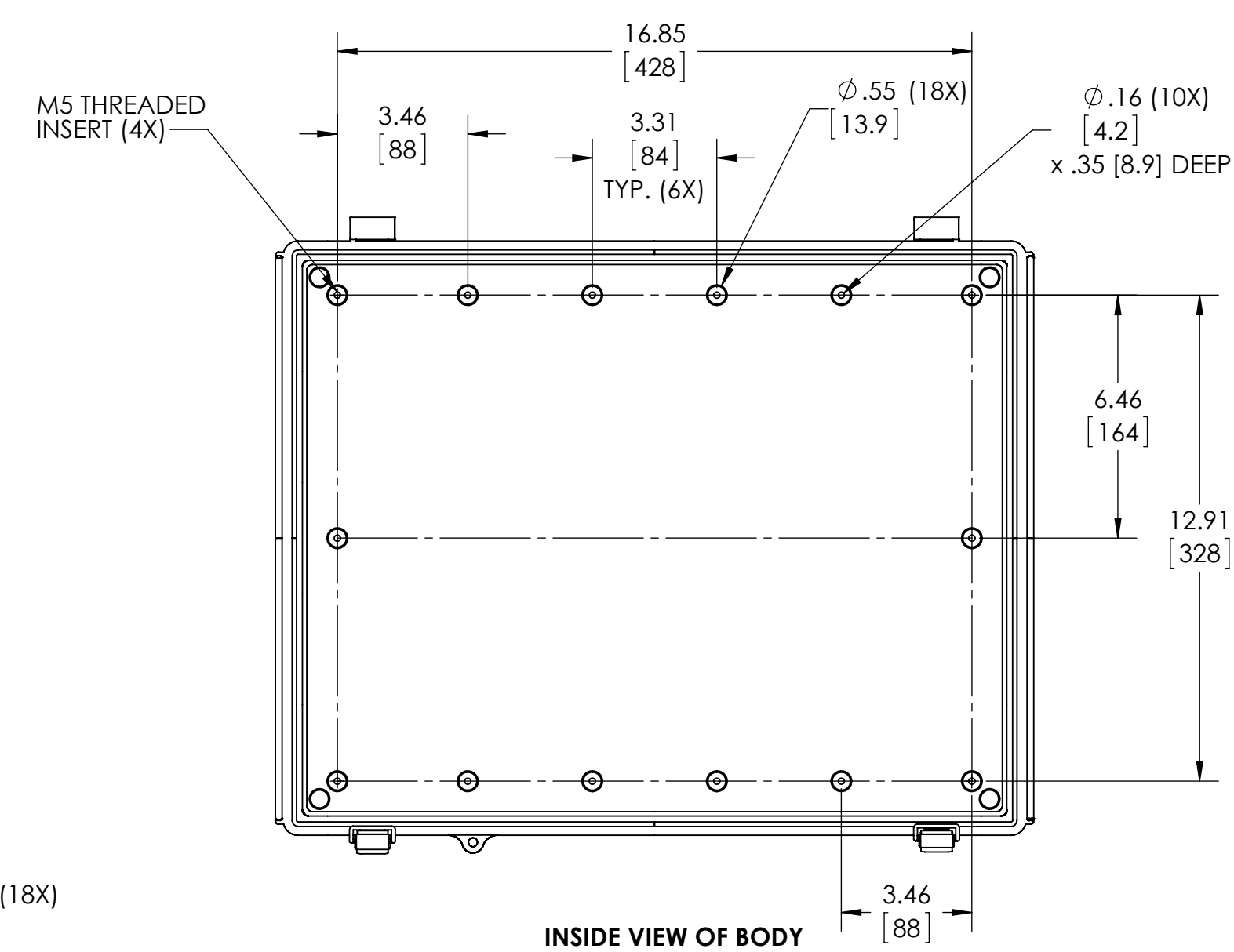
INSIDE VIEW OF BODY
