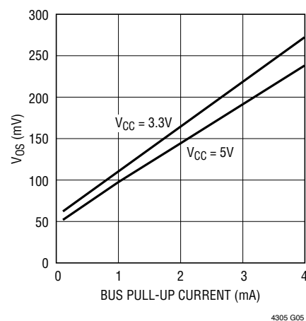
V_{OS,DOWN-BUF} vs Bus Pull-Up Current
