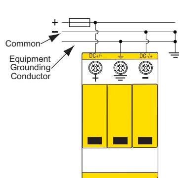
Application B 600Vdc systems only
