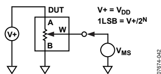
Figure 59. Potentiometer Divider Nonlinearity Error (INL, DNL)
