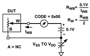
Figure 60. Wiper Resistance
