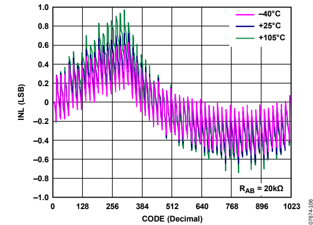
Figure 6. R-INL in R-Perf Mode vs. Code vs. Temperature (AD5292)
