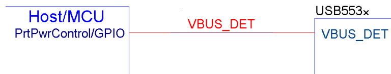
Figure 2.4 Embedded VBUS_DET Connection
