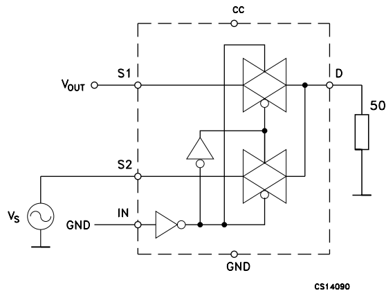
Figure 7. Test circuits
