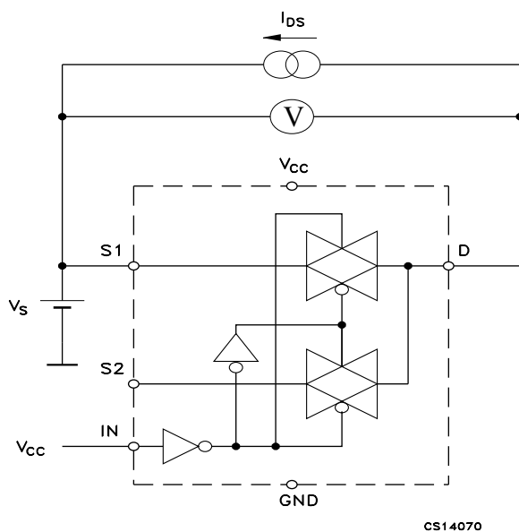
Figure 3. On-resistance
