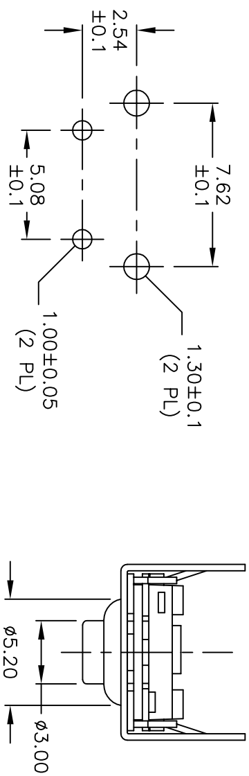
RECOMMENDED P.C.B. LAYOUT
