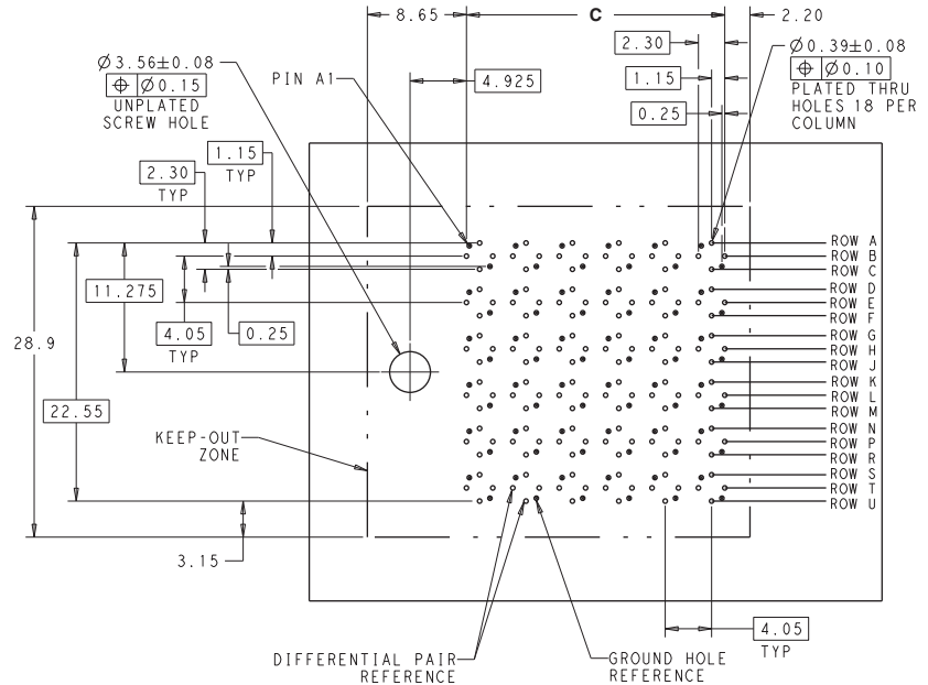
Left Guided Backplane Hole Pattern (Connector Side)
