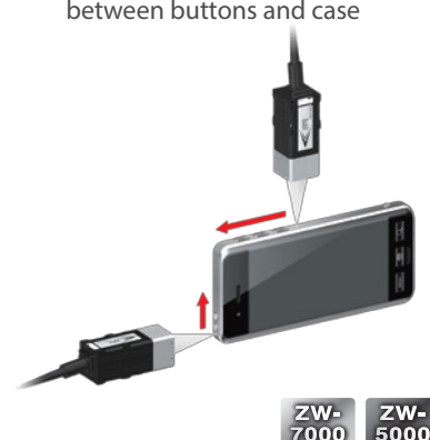
Level difference measurement between buttons and case
