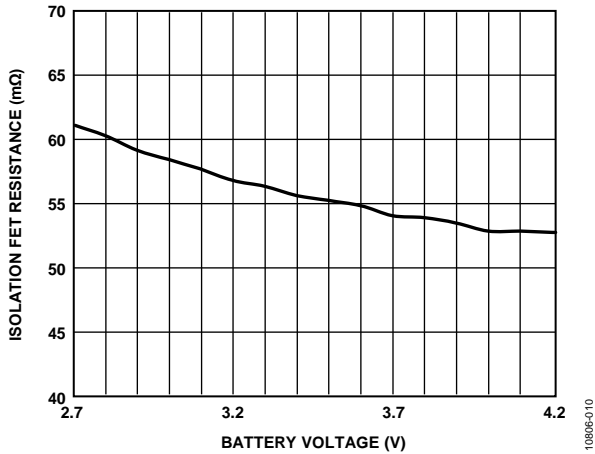
Figure 10. Ideal Diode R_{ON} vs. Battery Voltage, I_{SO\_Sk} = 500 mA, V_{INx} Open
