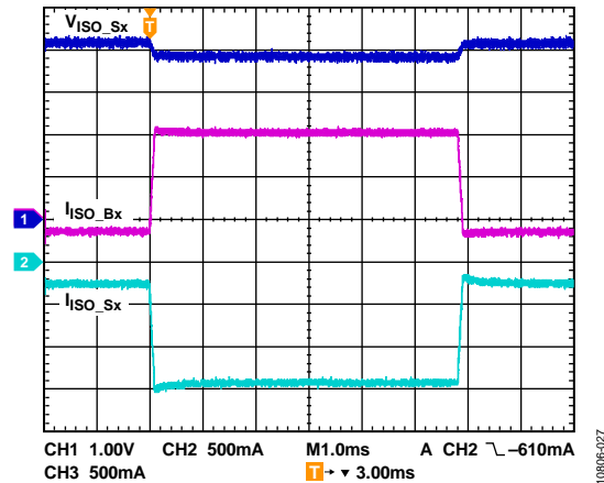
Figure 27. Load Transient, ISO_Sx Load = 300 mA to 1500 mA to 300 mA, EN\_CHG = \text{High} , ILIM[3:0] = 0110 (Binary) = 500 mA
