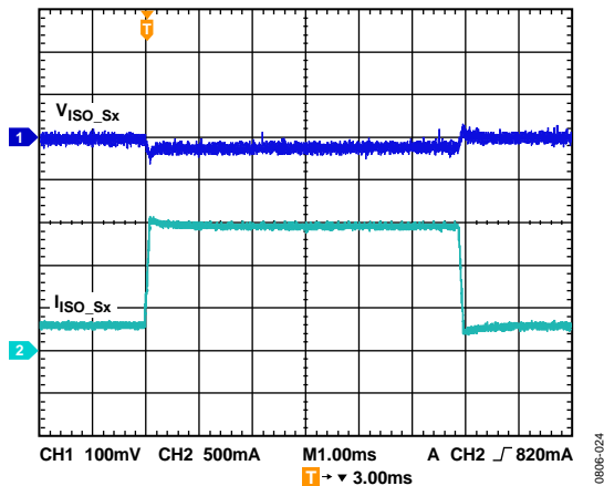
Figure 24. Load Transient, ISO_Sx Load = 300 mA to 1500 mA to 300 mA
