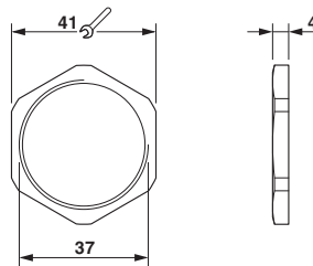
Dimensional drawing
