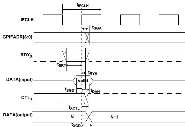
Figure 18. GPIF Synchronous Signals Timing Diagram
