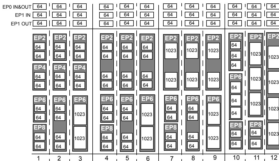
Figure 6. Endpoint Configuration
