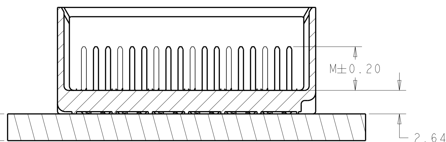
SECTION Z-Z
