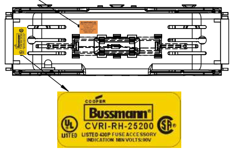
RM25200-1CR WITH CVRI-RH-25200 INSTALLED
