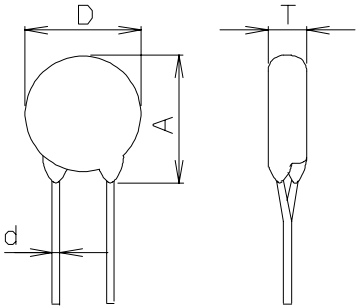
Fig. 1.1 Straight Leads and Taping
