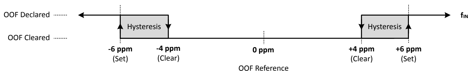
Figure 3.13. Example of Precise OOF Monitor Assertion and De-assertion Triggers
