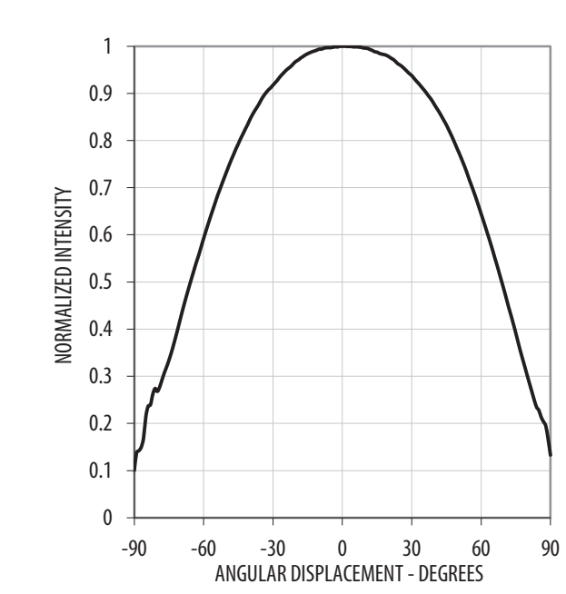
Figure 5: Radiation Pattern
