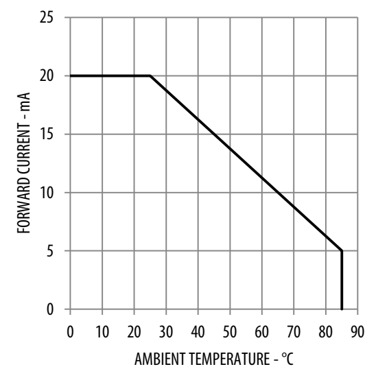
Figure 10: Derating Curve
