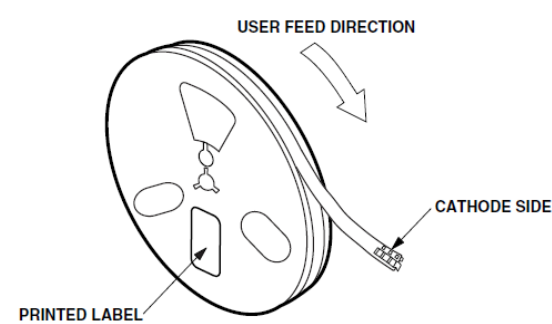
Figure 12: Reel Orientation
