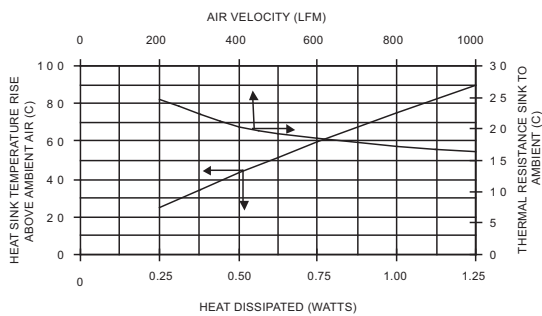
NATURAL AND FORCED CONVECTION CHARACTERISTICS
