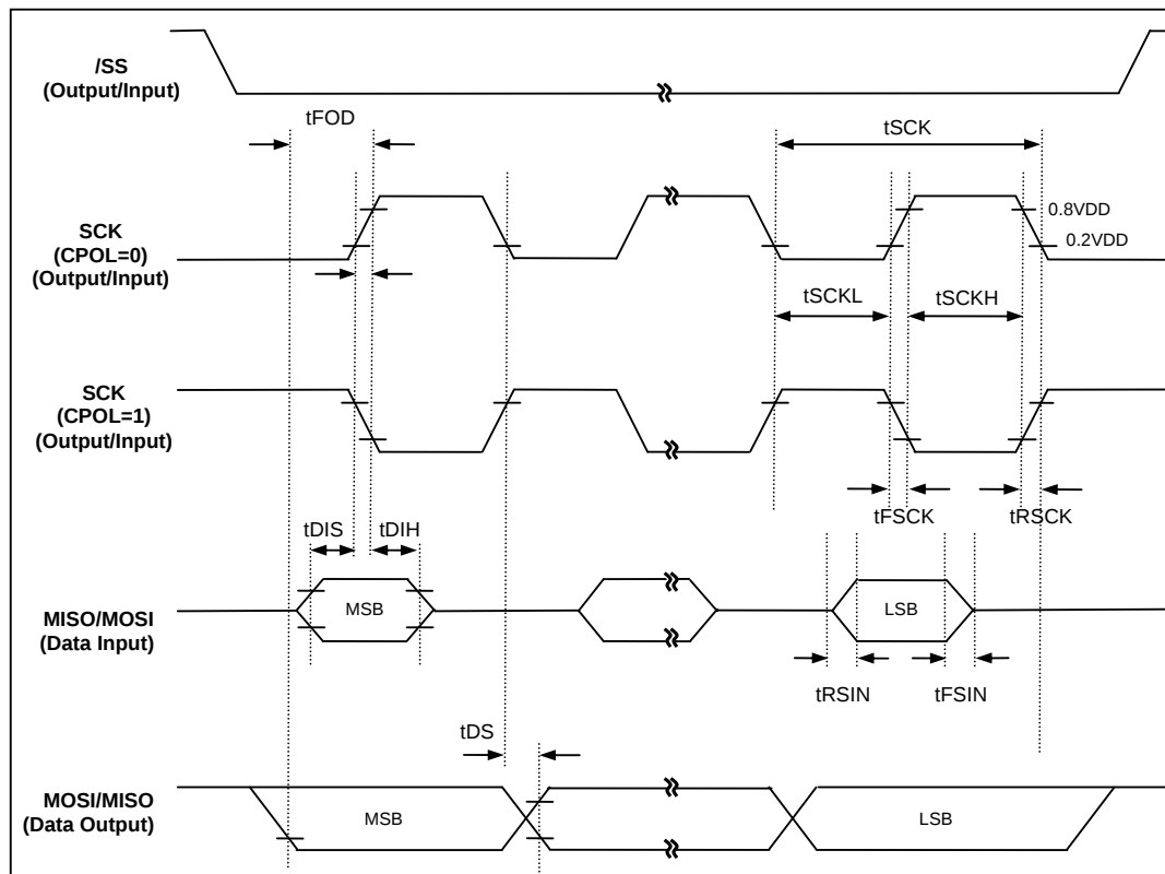
Figure 7-2 SPI Timing
