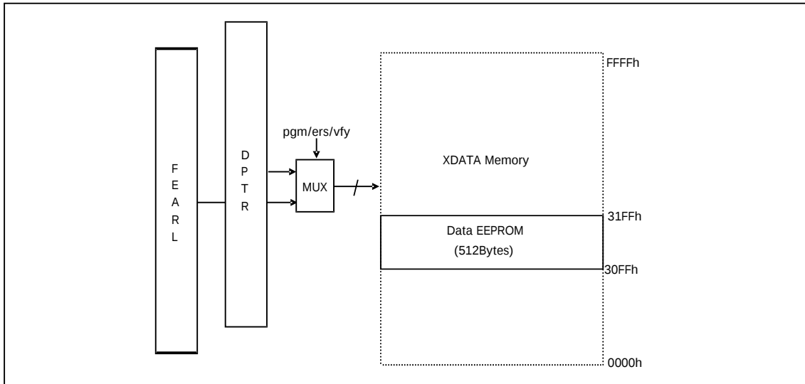
Figure 15-3 Data EEPROM memory map
