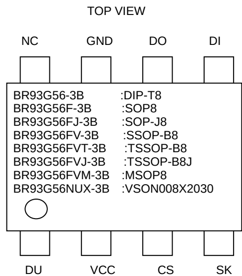
Figure 3. Pin Configuration
