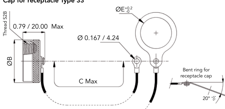
Cap for receptacle Type 33
