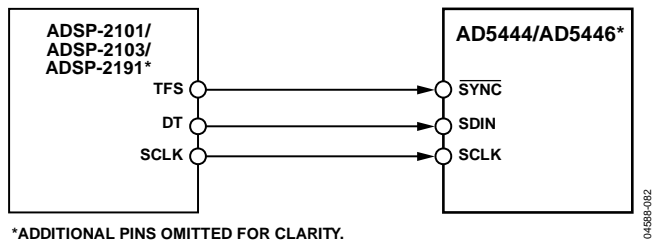
*ADDITIONAL PINS OMITTED FOR CLARITY. 04688-082
