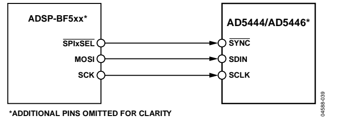
*ADDITIONAL PINS OMITTED FOR CLARITY. 04688-039
