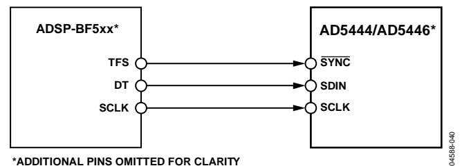
*ADDITIONAL PINS OMITTED FOR CLARITY. 04688-040
