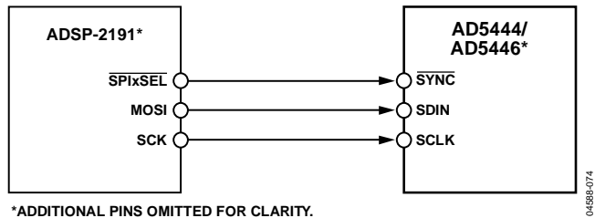
*ADDITIONAL PINS OMITTED FOR CLARITY. 04688-074
