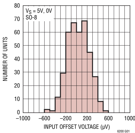
V_{OS} Distribution, V_{CM} = V^+/2
