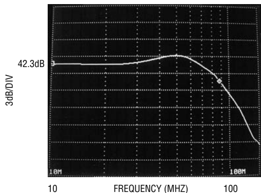
Instrumentation Amplifier Frequency Response
