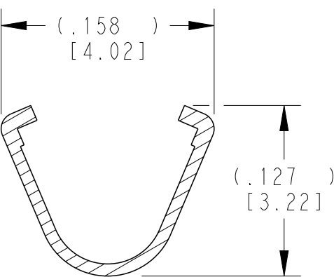
SECTION A-A WIRE BARREL
