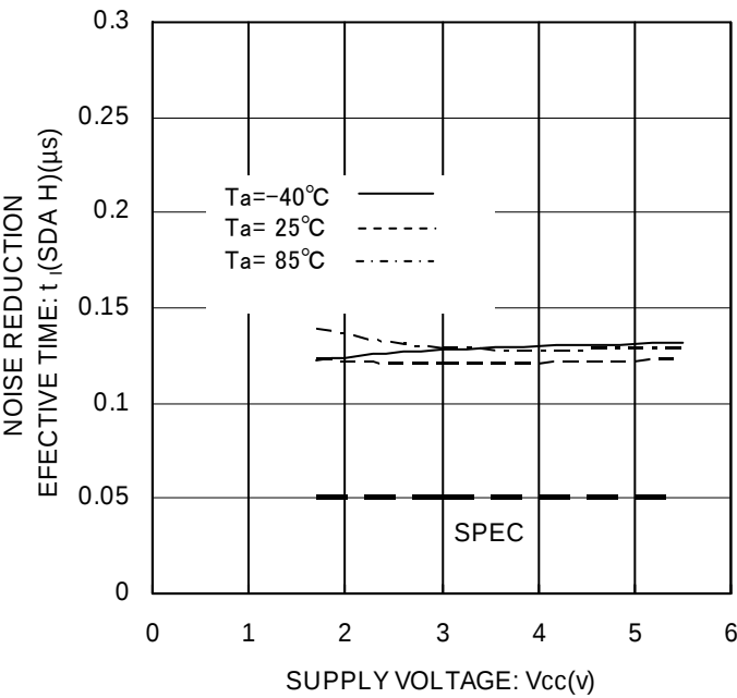
Figure 30. Noise Spike Width t_I (SDA H)
