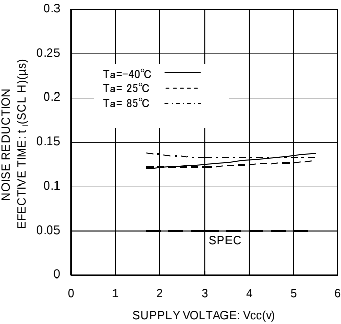
Figure 28. Noise Spike Width t_I (SCL H)
