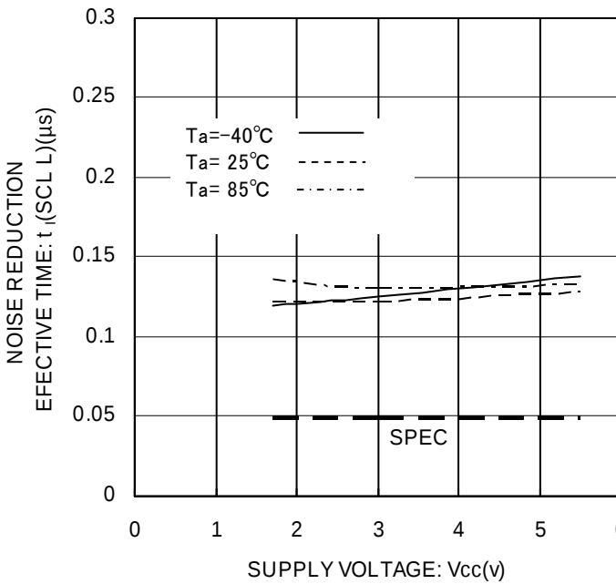
Figure 29. Noise Spike Width t_I (SCL L)
