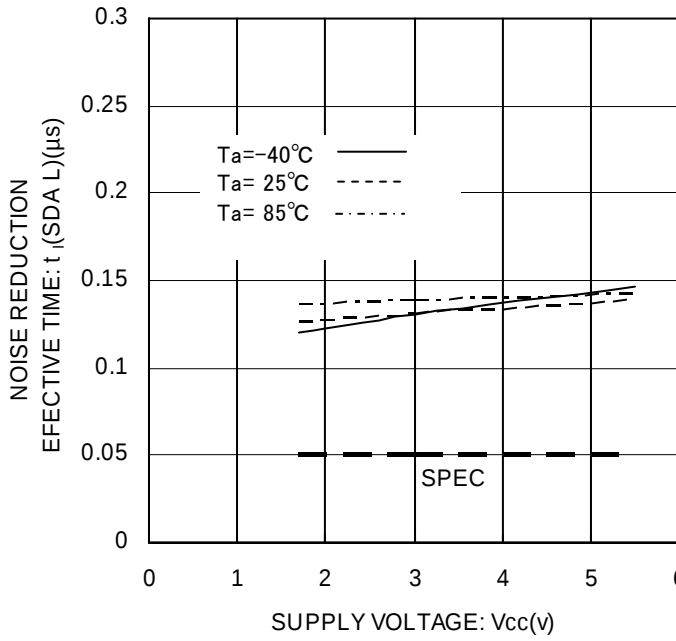
Figure 31. Noise Spike Width t_I (SDA L)
