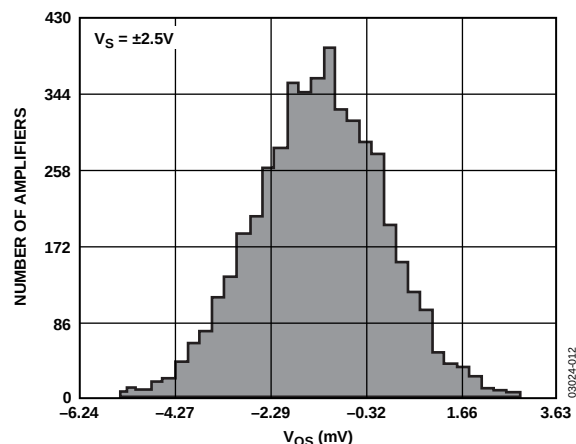
Figure 12. V_{OS} Distribution
