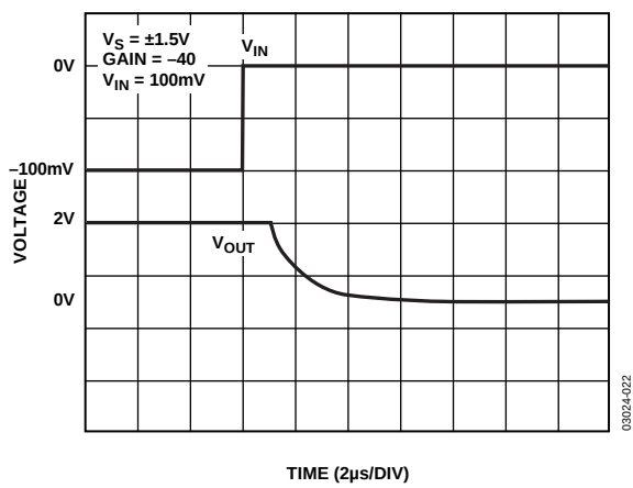
Figure 22. Saturation Recovery
