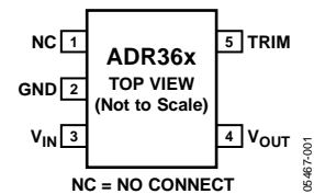
Figure 1.5-Lead TSOT (UJ)
