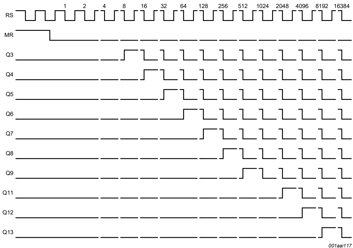
Fig. 7. Timing diagram
